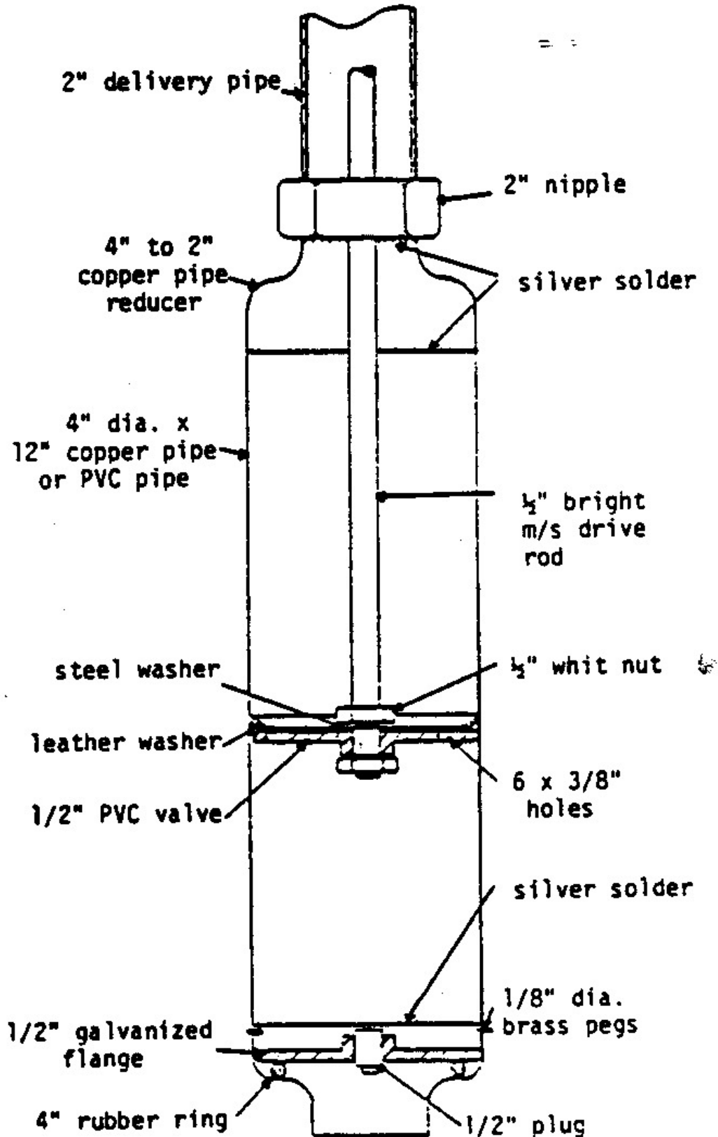
(Bilge Pump Configuration)
